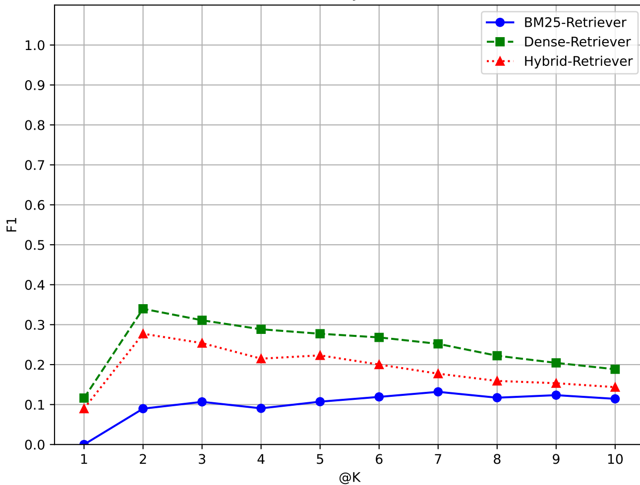
Query 33
